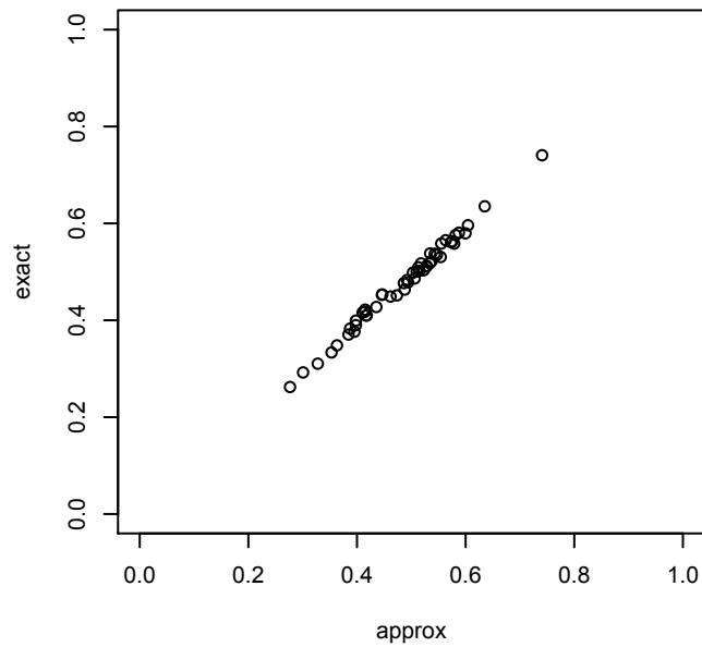
chunks=3, L=10
