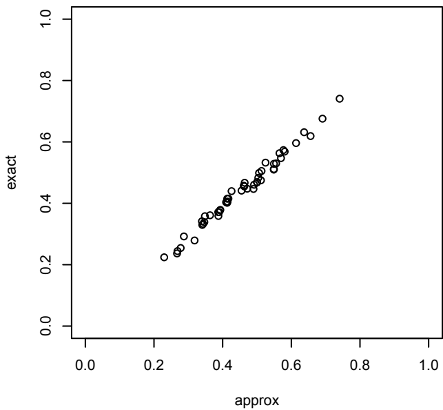
chunks=3, L=5
